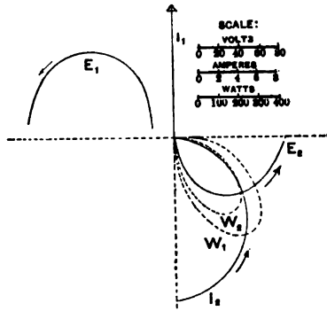
FIG. 9.—Constant Current, Step Down, Arm at 150°
